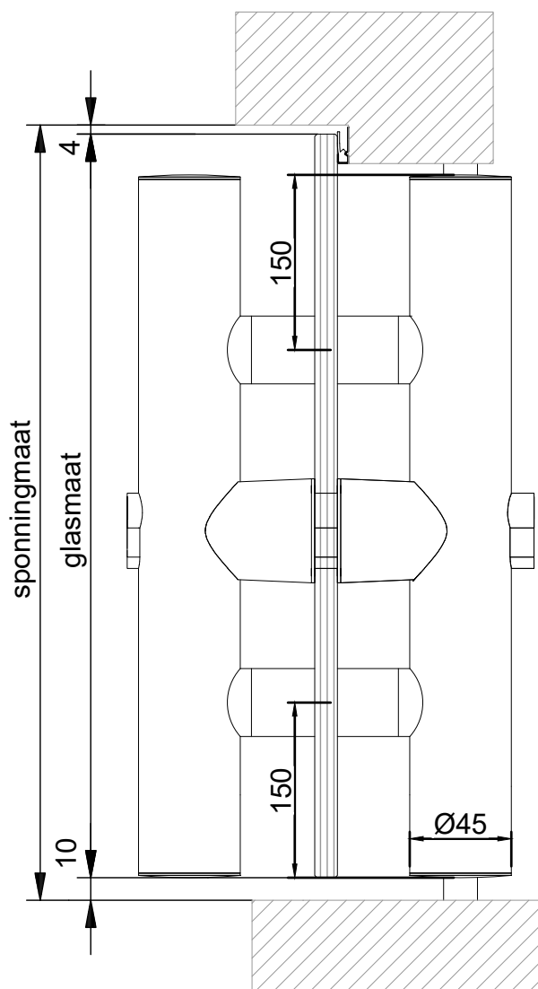
VERTICALE DOORSNEDE type TGD-1D
