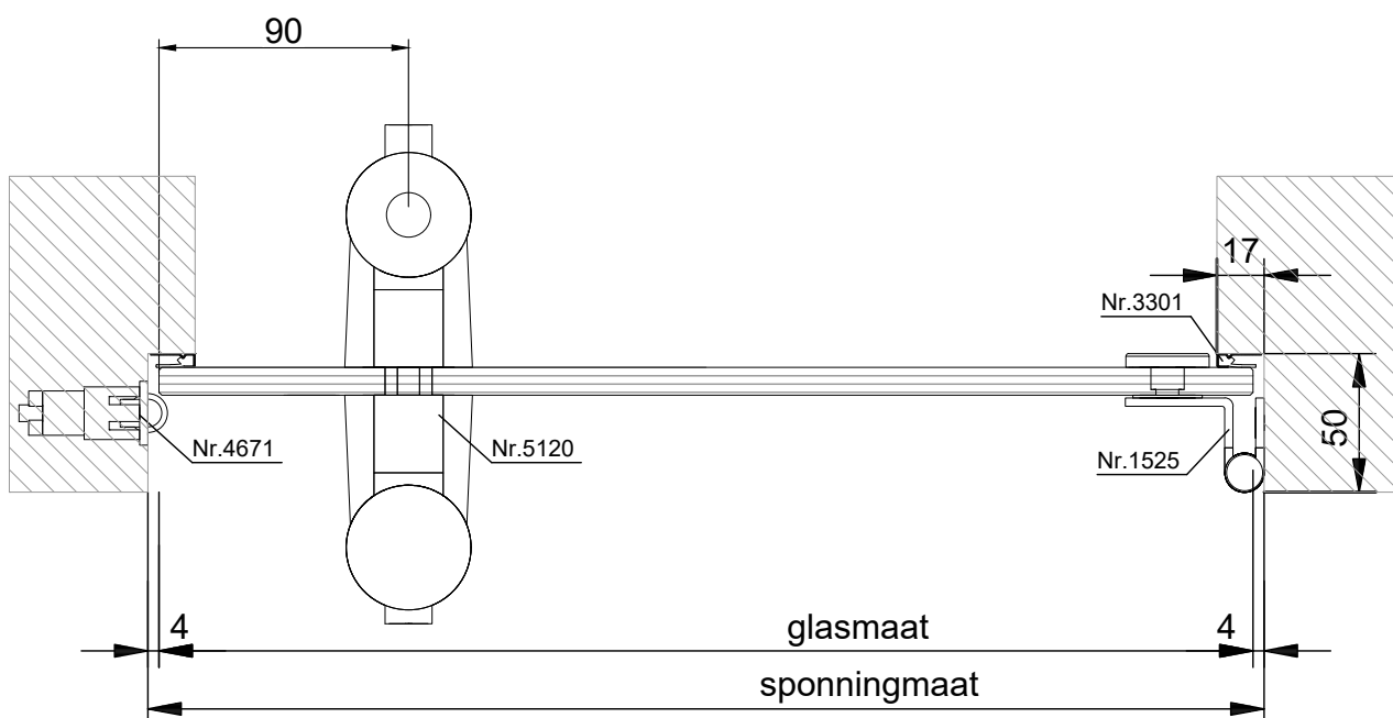
HORIZONTALE DOORSNEDE type TGD-1D
