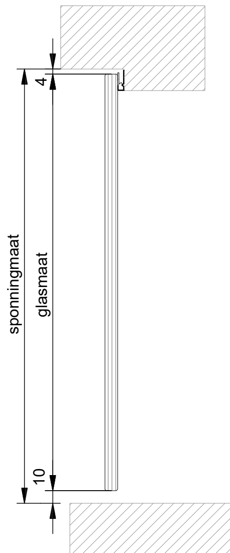
VERTICALE DOORSNEDE type TGD-1B
