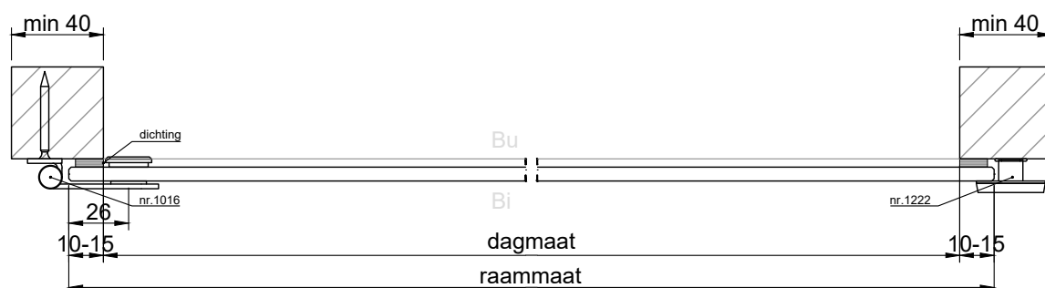
HORIZONTALE DOORSNEDE type DVR-5
