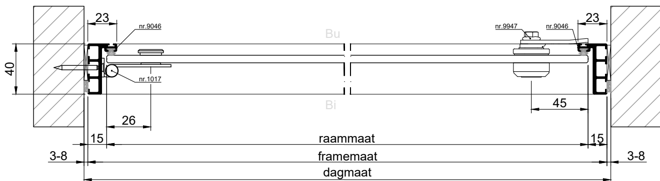
HORIZONTALE DOORSNEDE type DVR-7
