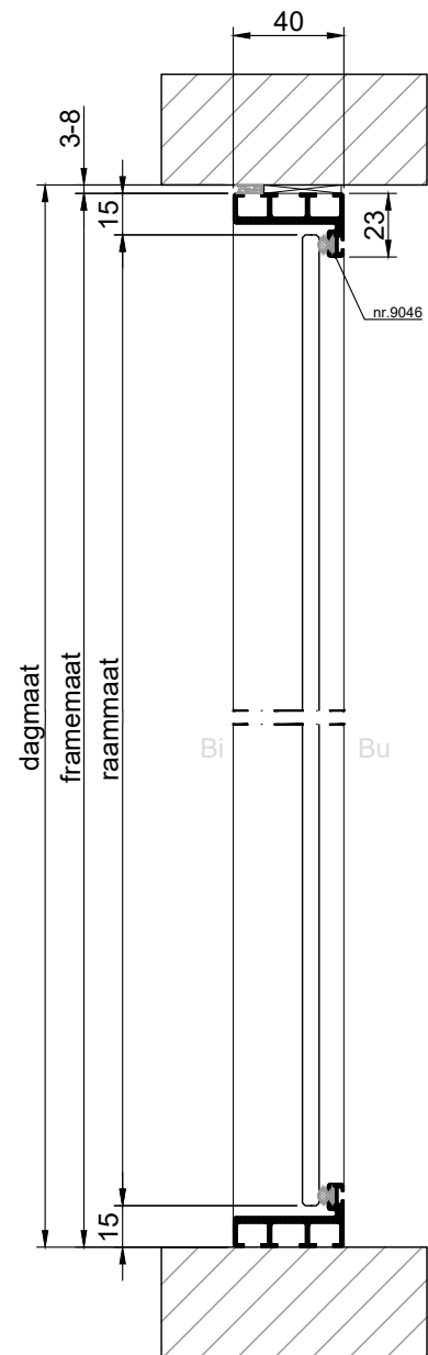
VERTICALE DOORSNEDE type DVR-7
