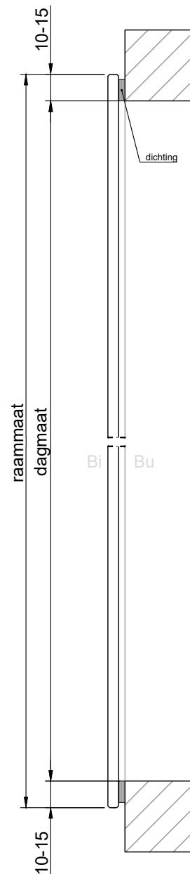
VERTICALE DOORSNEDE type DVR-5
