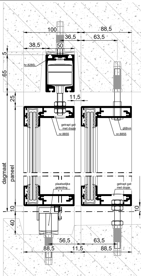
VERTICALE DOORSNEDE type BSH-10C
