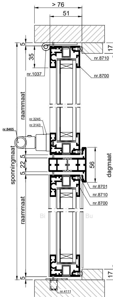
VERTICALE DOORSNEDE type AMC-40
