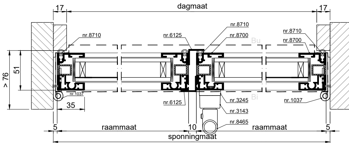
HORIZONTALE DOORSNEDE type AMC-40
