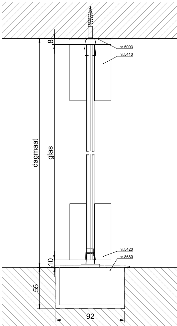
VERTICALE DOORSNEDE type TPM-1D
