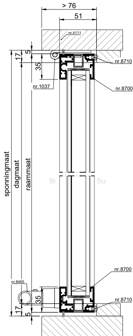
VERTICALE DOORSNEDE type AMK-20
