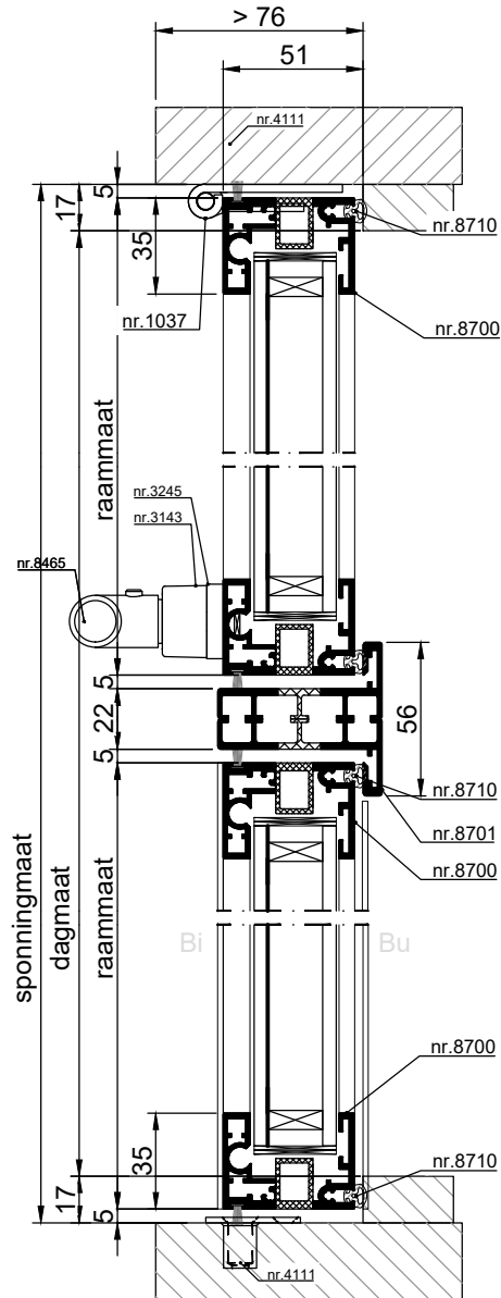
VERTICALE DOORSNEDE type AMC-40
