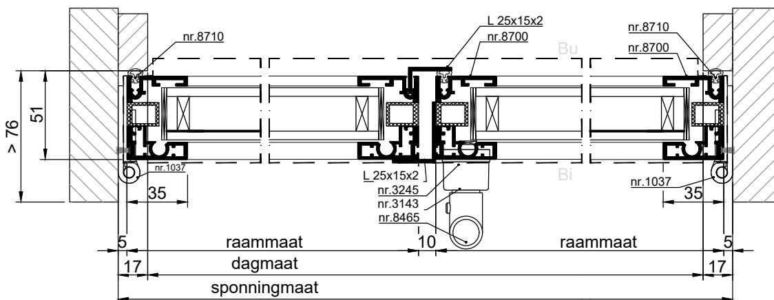
HORIZONTALE DOORSNEDE type AMC-40
