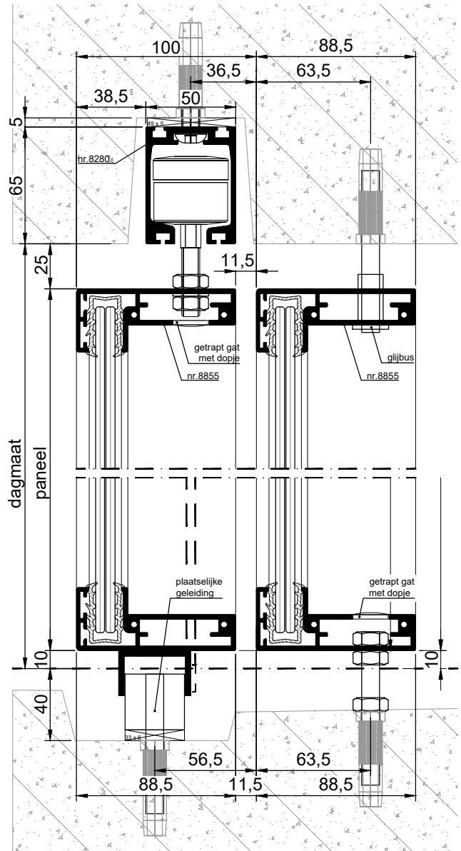
VERTICALE DOORSNEDE type BSH-10C
